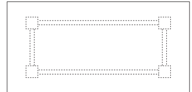
NC-017-240 W2400 × D1200 × H720
