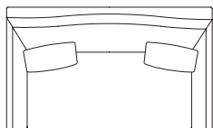
NC-046BC/C-2P W1500 × D900 × H850(SH400)AH650
