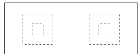
NC-029A-300 W3000 × D1200 × H720
