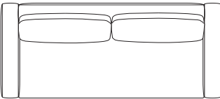
MD-805-3P W2100・D900・H750 (SH380)AH530
