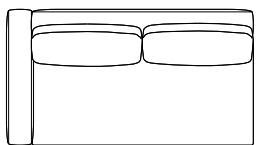
MD-805-2PR/2PL W1635・D900・H750 (SH380)AH530 (図面はMD-805-2PR右肘)
