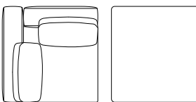
MD-805-CRR/CRL W900・D900・H750 (SH380)AH530 (図面はMD-805-CRR)
