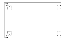
AD-892A / AD-892B (135T) W1350・D800・H700 (t 30)
