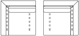
MD-1105-CRR W900-D900-H760 (SH380) MD-1105-CRL W900-D900-H760 (SH380)
