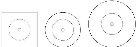
AD-898HL(90) W900・D900・H700(t 25) AD-898HL(90C) φ900・H700(t 25) AD-898HL(120C) φ1200・H700(t 25)
