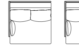
AD-085B-1P W960-D930-H750-SH400
