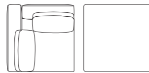
MD-805-CRR/CRL W900×D900×H750 (SH380) AH530 (図面はMD-805-CRR)
