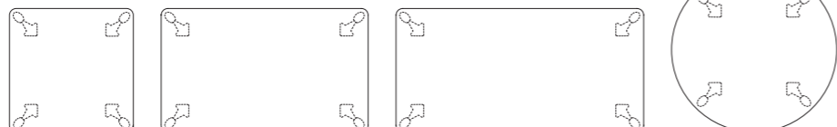
AD-152 (90) W900-D900-H700 (t 35) AD-152 (150) W1500-D900-H700 (t 35) AD-152 (180) W1800-D900-H700 (t 35) AD-152 (120) φ1200-H700 (t 35)
