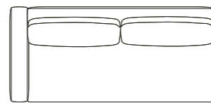
MD-805-3PR/3PL W1935×D900×H750 (SH380) AH530 (図面はMD-805-3PR右肘)
