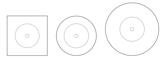
AD-898HL(90) W900-D900-H700(t 25) AD-898HL(90C) φ900-H700(t 25) AD-898HL(120C) φ1200-H700(t 25)
