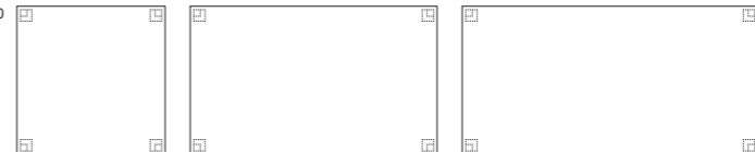
AD-885 (90) W900-D900-H700 (t 45) AD-885 (150) W1500-D900-H700 (t 45) AD-885 (180) W1800-D900-H700 (t 45)
