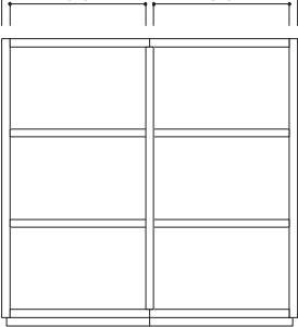
MD-302W / WL W1800-D400-H1750
