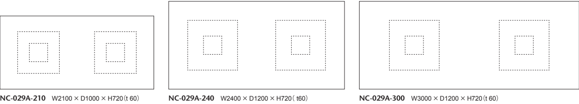
NC-029A-210 W2100 × D1000 × H720 (t 60)
