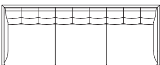
NC-026 W2100 × D800 × H750 (SH420)
