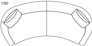
MD-3211-3PL W2100-D1035-H790 (SH400) (クッション×2)
