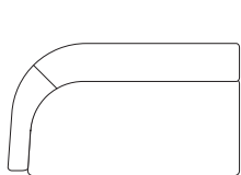
MD-3211-2PR/2PL W1400-D800-H710 (SH400)
