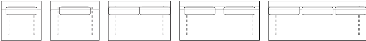
MD-1105-S-90 W900-D900-H760 (SH380) MD-1105-S-110 W1100-D900-H760 (SH380) MD-1105-S-140 W1400-D900-H760 (SH380) MD-1105-S-180 W1800-D900-H760 (SH380) MD-1105-S-220 W2200-D900-H760 (SH380)
