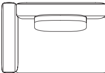
AD-229-2PSR / 2PSL W1400・D950・H770 (SH380)・AH650 (図はAD-229-2PSR)
