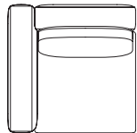
AD-229-1PR / 1PL W950・D950・H770 (SH380)・AH650 (図はAD-229-1PR)
