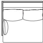
AD-085BR-BL-1P W930-D930-H750-SH400
