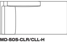
MD-505-CLR/CLL-H W733・D1500・H960 (SH400)・AH600 (図はMD-505-CLL-H左肘)
