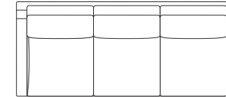
MD-505-3PR/3PL-H W2000・D900・H960 (SH400)・AH600 (図はMD-505-3PR-H右肘)
