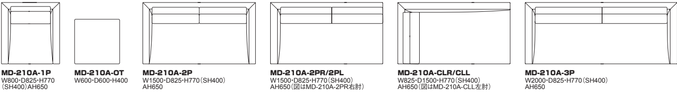
MD-210A-1P W800・D825・H770 (SH400) AH650 MD-210A-OT W600・D600・H400 MD-210A-2P W1500・D825・H770 (SH400) AH650 (図はMD-210A-2PR右肘) MD-210A-2PR/2PL W1500・D825・H770 (SH400) AH650 (図はMD-210A-2PR右肘) MD-210A-CLR/CLL W825・D1500・H770 (SH400) AH650 (図はMD-210A-CLL左肘) MD-210A-3P W2000・D825・H770 (SH400) AH650
