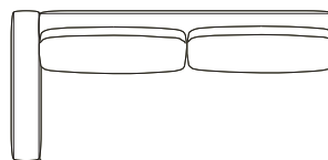
MD-805-3PR/3PL W1935・D900・H750 (SH380)AH530 (図面はMD-805-3PR右肘)
