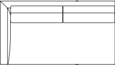
MD-210A-2PR/2PL W1500・D825・H770 (SH400) AH650 (図はMD-210A-2PR右肘)
