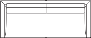
MD-210A-3P W2000・D825・H770 (SH400) AH650
