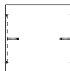
MD-1203 W/G-AL-90S W900・D900・H350
