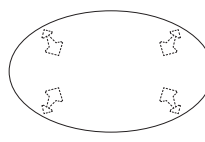
AD-892A / AD-892B (135T) W1350・D800・H700 (t 30)
