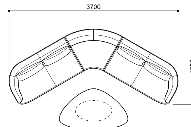
NC-075-2P-SR+C60+2P-SL MD-3212W-150T
