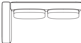
AD-229-2PR / 2PL W1800・D950・H770 (SH380)・AH650 (図はAD-229-2PR)
