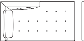
MD-705-CLR/CLL W850・D1600・H850 (SH400)・AH720 (図面はMD-705-CLL左肘)
