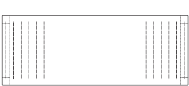
AD-026 (240) W2400・D900・H720 (t 60)
