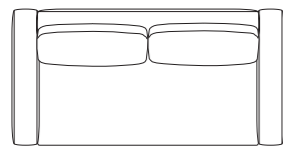
MD-805-2P W1800×D900×H750 (SH380) AH530
