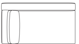
MD-805-CLR/CLL W900×D1635×H750 (SH380) AH530 (図面はMD-805-CLL左肘)
