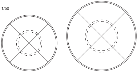
MD-1302N-120 φ1200・H720 (脚部φ550)
