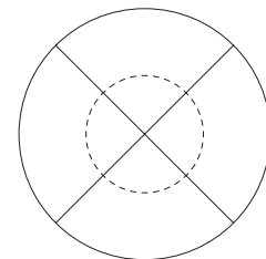
AD-033HL 150C: φ1500・H700 (t 30)
