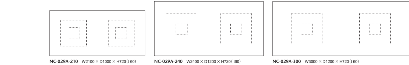
NC-029A-210 W2100 × D1000 × H720 (t 60)
