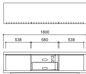
MD-301N-180 W1800×D450×H500
