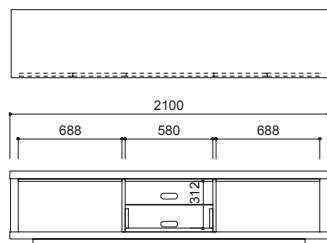
MD-301N-210 W2100×D450×H500
